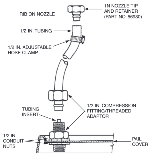
FIGURE 4 000367
