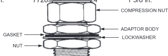
FIGURE 19 000154
