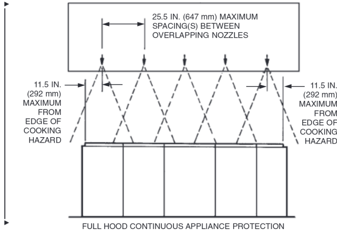
FIGURE 75 007538
