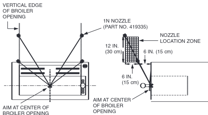
FIGURE 49 007128
