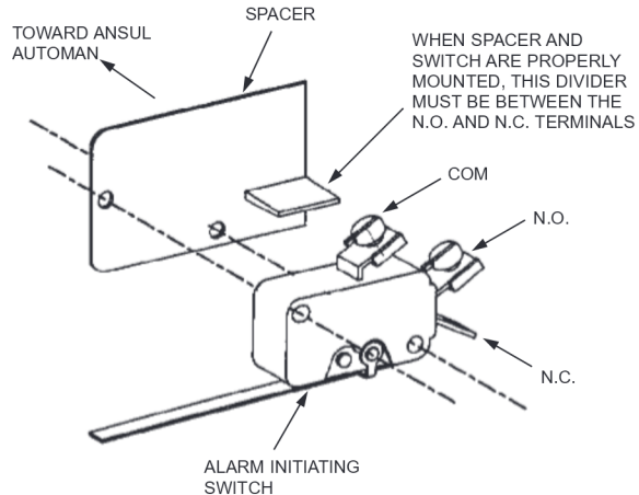
FIGURE 30 004890
