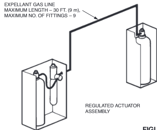
FIGURE 11 000777
