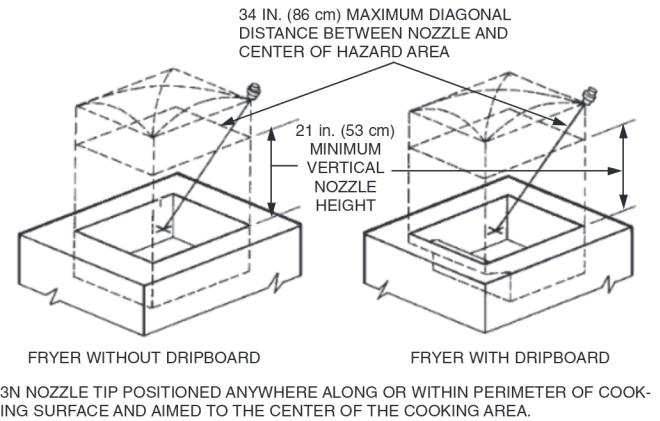
FIGURE 18 002287
