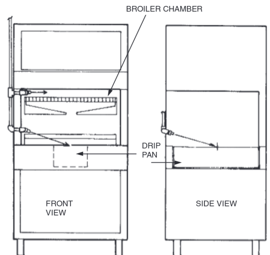
FIGURE 50 000252
