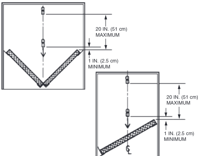
FIGURE 7 000199
