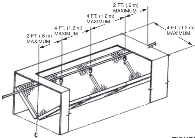
FIGURE 6 000197
