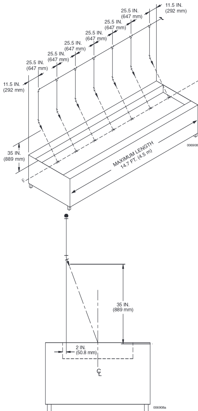
FIGURE 71
