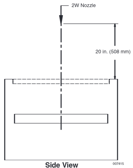
FIGURE 63c
