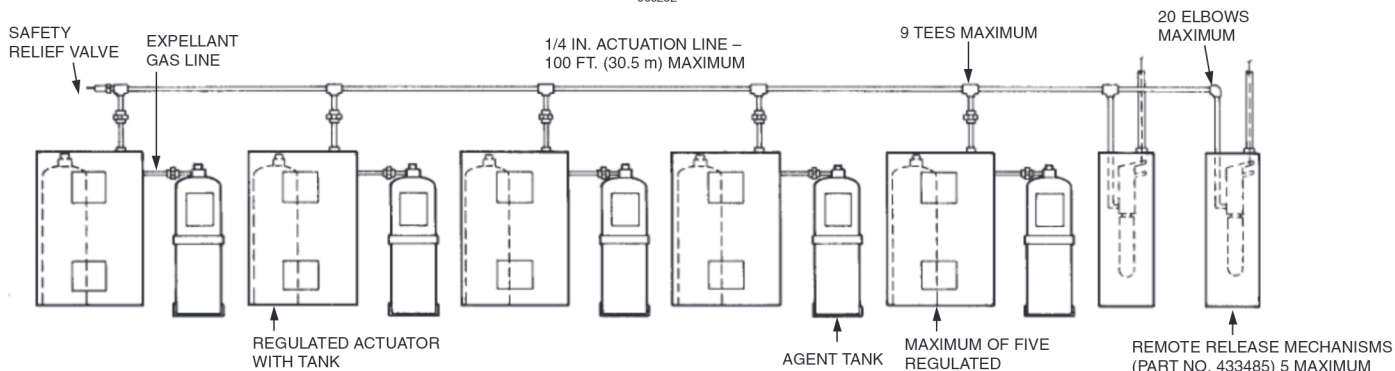
FIGURE 81 000262
