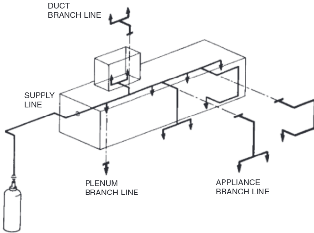
FIGURE 86
