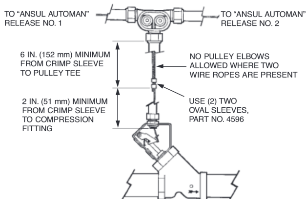
FIGURE 64 001091
