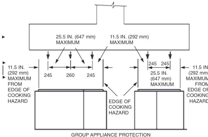
FIGURE 76 001720
