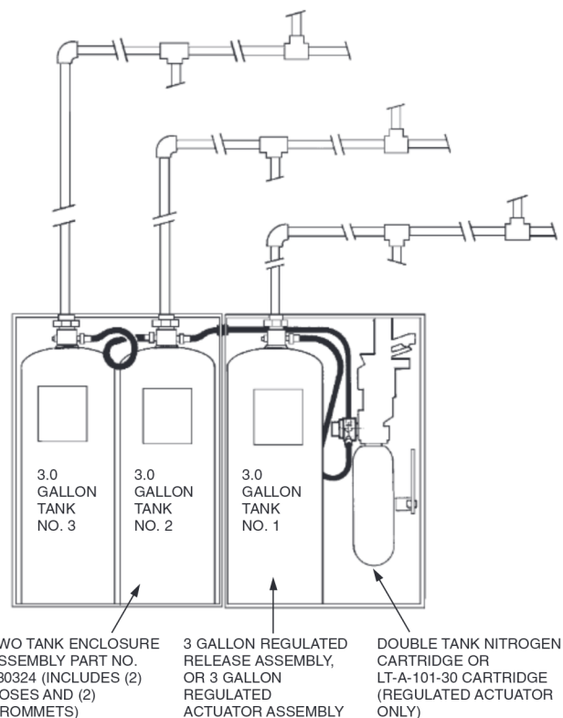
FIGURE 97 000007
