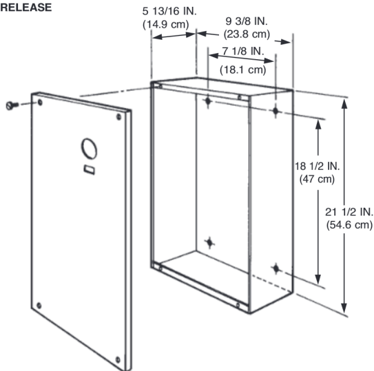
FIGURE 4a 000464
