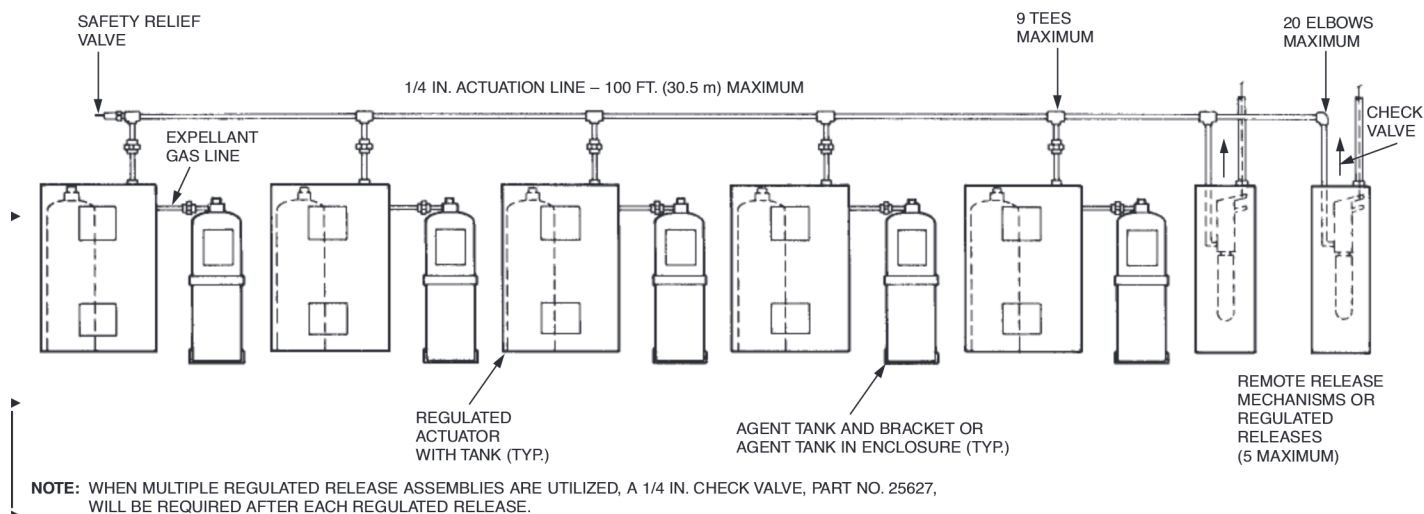
FIGURE 12 000301
