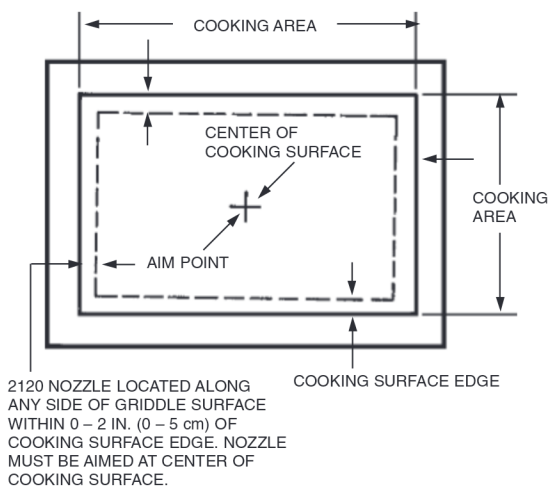
FIGURE 44 000241
