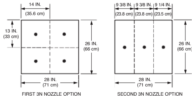
FIGURE 1 002466
