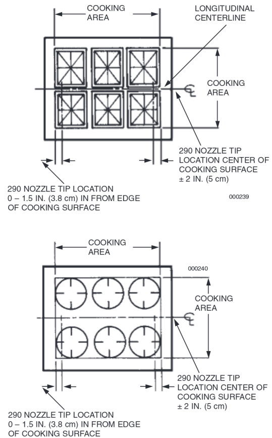
FIGURE 34
