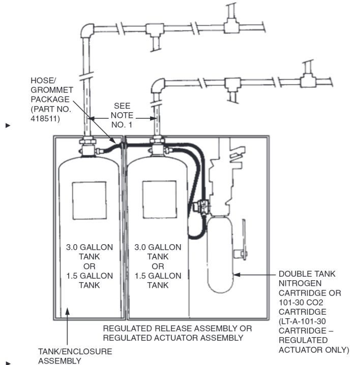
FIGURE 96 000786
