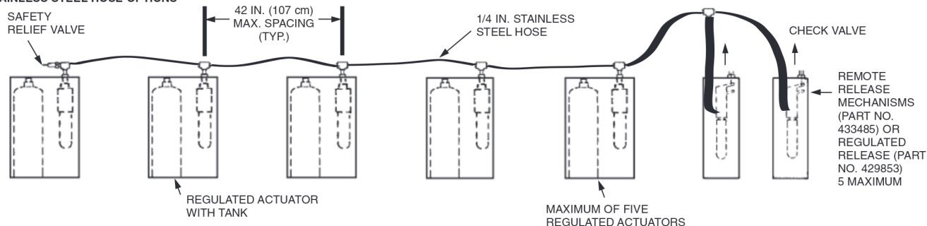
FIGURE 82 000301
