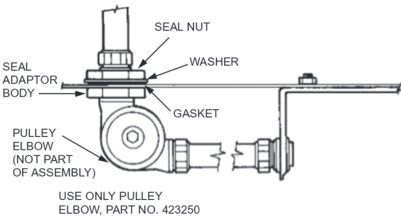
FIGURE 21 000156
