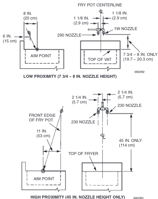
FIGURE 58
