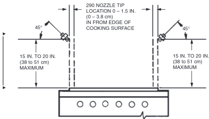
FIGURE 33 002276
