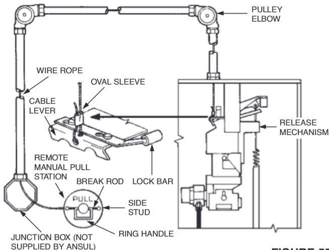
FIGURE 55 001090
