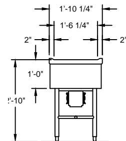
END VIEW
