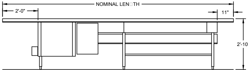
TR-10 ELEVATION VIEW
