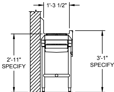
Typical Section View at Tray-Drop
