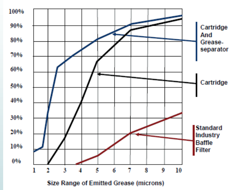
Figure 1a grease removal efficiency chart
